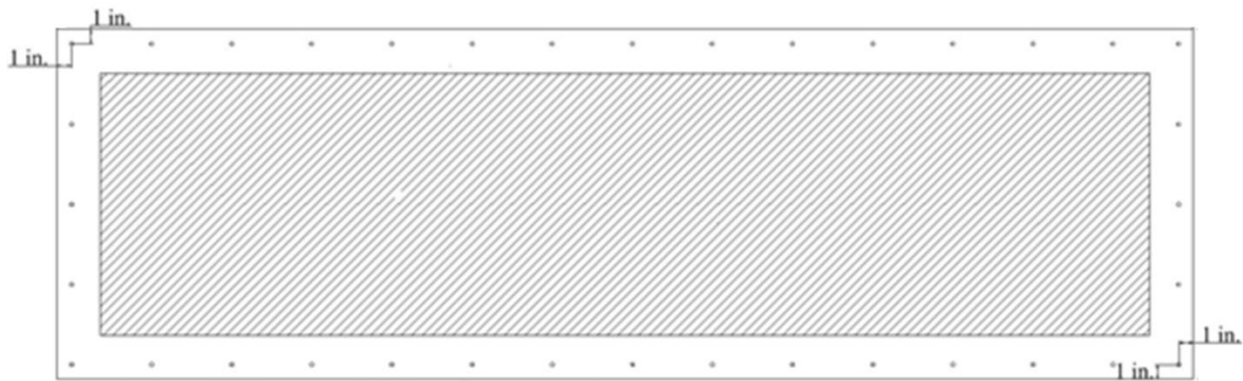
Fastening Pattern for Attachment of TAMCO 4ft Tile Off-Ridge Vent
